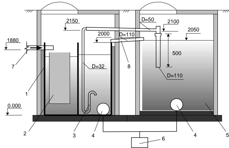
Plan of separation surplus active sediments from «BIOTAL- 4»
