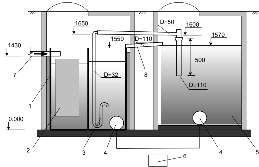
Plan of separation surplus active sediments from «BIOTAL- 2» 1 - BIOTAL-2; 2 - intake chamber; 3 - airlift for pumping of superfluous active sediments; 4 - aerators; 5 - tank for superfluous sediments; 6 - compressor; 7 - inflow of waste water; 8 - outflow of sediment water.
